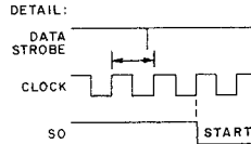
Fig.27 UAR/T-TRANSMITTER TIMING
