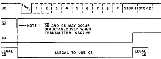
Fig.8 ALLOWABLE POINTS TO USE CONTROL STROBE
